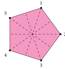
fr^4 = r f
