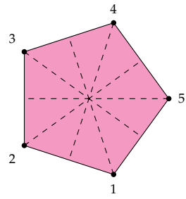
fr = r^4 f
